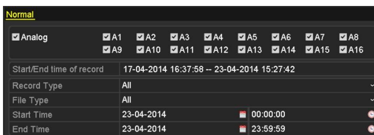
Figura 5. 29 Export
