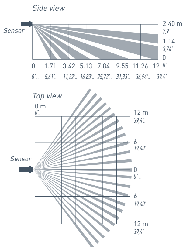
PICTURE 3. Sensor's detection zone
